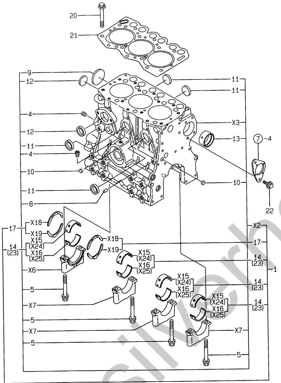
Fia.1.CYLINDER BLOCK 1.CYLINDER BLOCK
