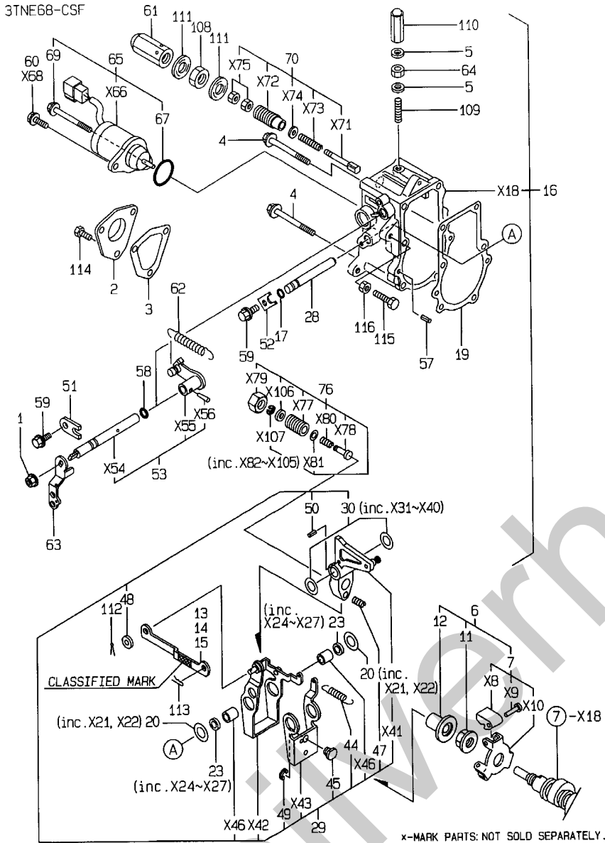
Fig.12.GOVERNOR 12. GOVERNOR
